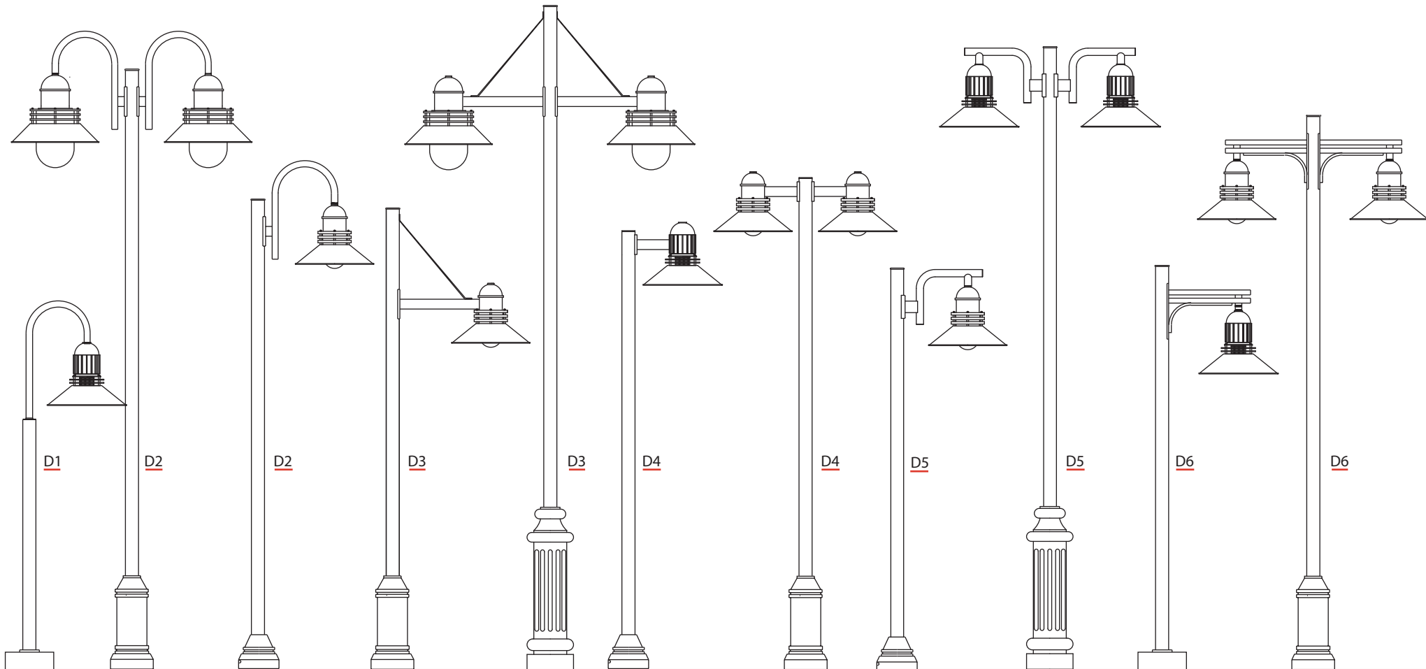
Bases, poles and mountings.
