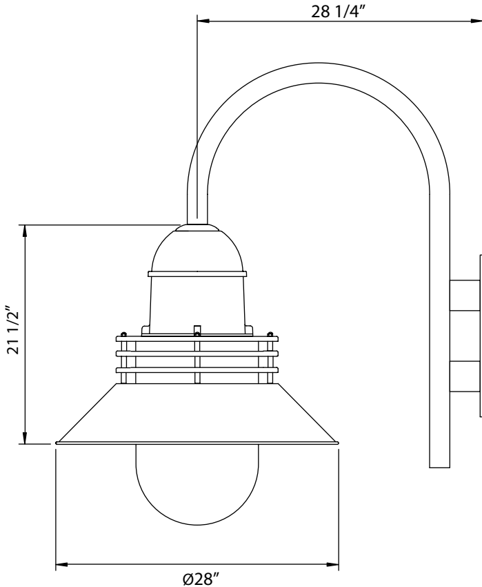
WMS mounting style
