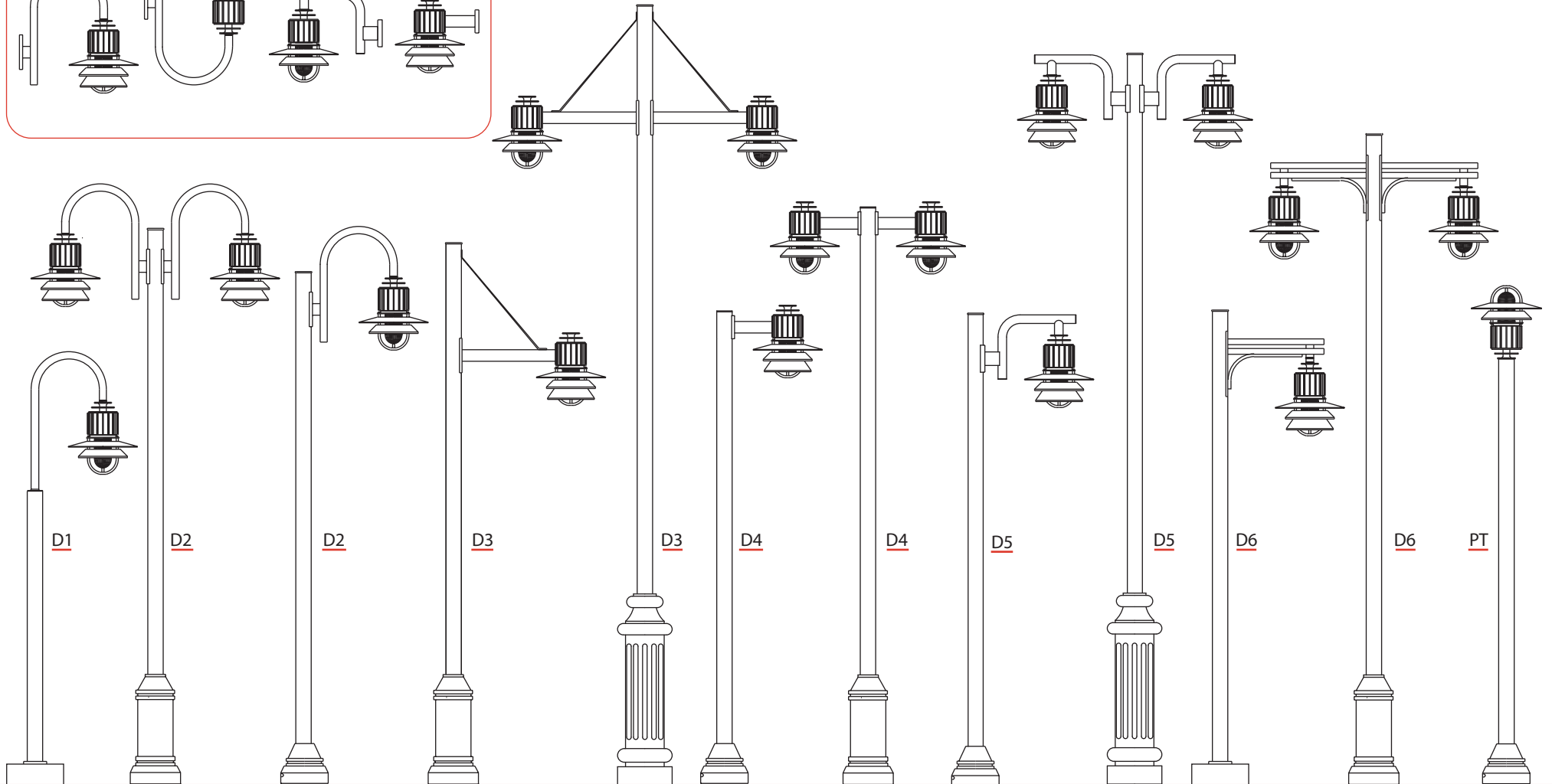
Bases, poles and mountings.
