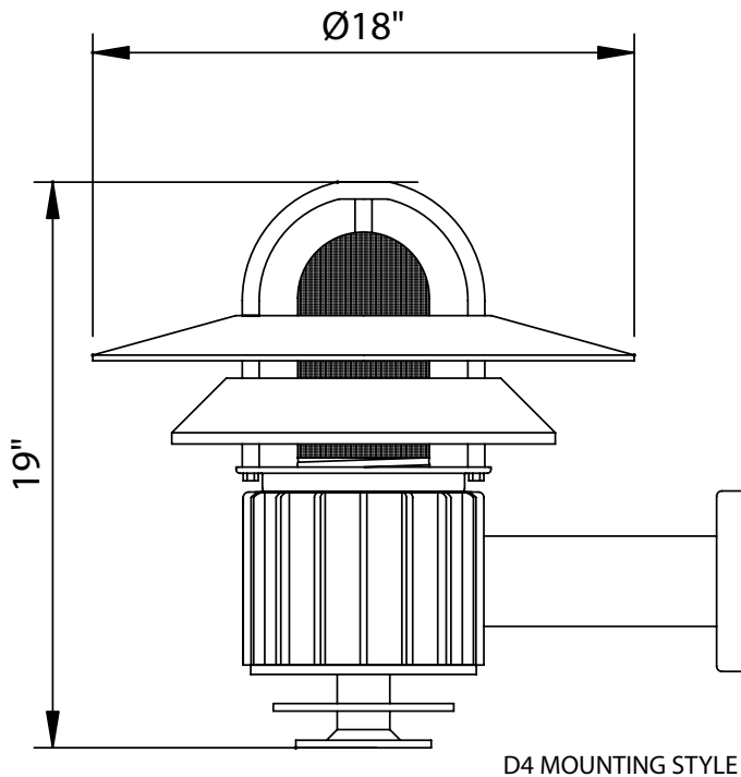
D4 MOUNTING STYLE
